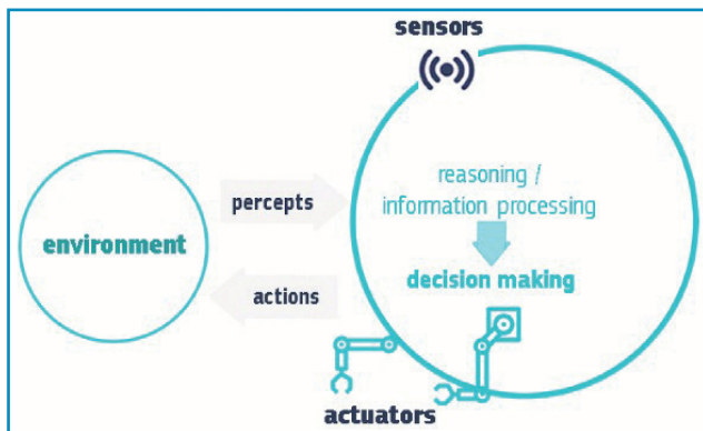
Figure 2: AI system
